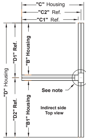
T9 - "T" Section
