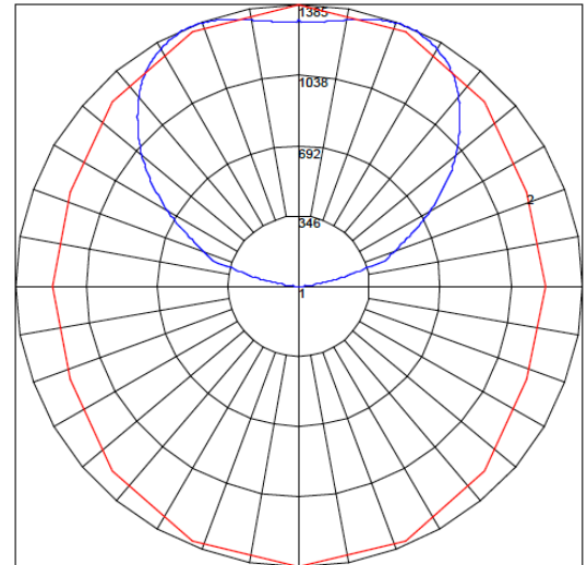
Maximum Candela = 1384.56 Located At Horizontal Angle = 90, Vertical Angle = 157.5 # 1 - Vertical Plane Through Horizontal Angles (90 - 270) (Through Max. Cd.) # 2 - Horizontal Cone Through Vertical Angle (157.5) (Through Max. Cd.)
