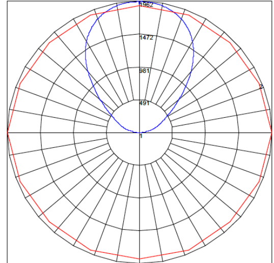
Maximum Candela = 1962 Located At Horizontal Angle = 0, Vertical Angle = 179 # 1 - Vertical Plane Through Horizontal Angles (0 - 180) (Through Max. Cd.) # 2 - Horizontal Cone Through Vertical Angle (179) (Through Max. Cd.)
